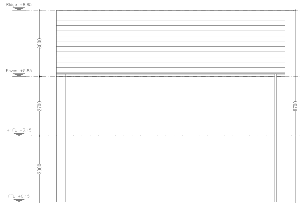
House Type N1 Semi-Detached Side Elevation
