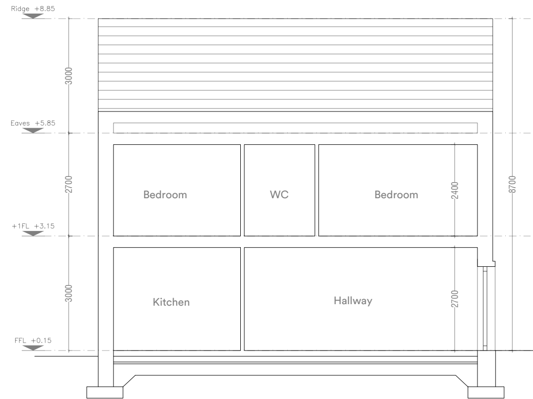
House Type N1 Semi-Detached Section A.A
